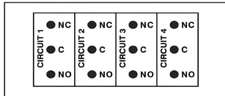
4-POLE WIRING DIAGRAM
