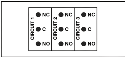
3-POLE WIRING DIAGRAM
