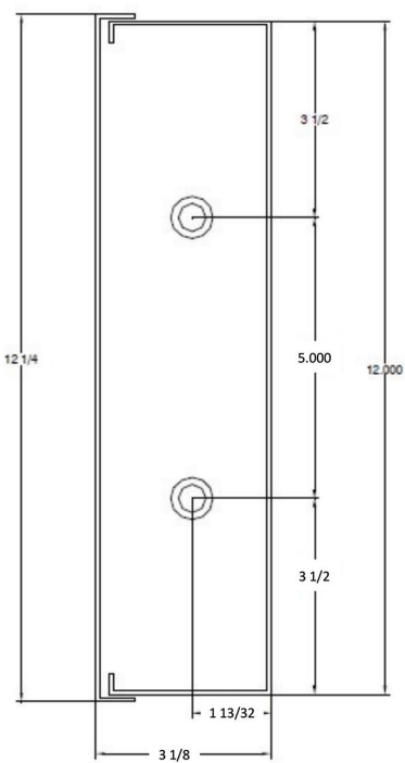
CBC Mounting Dimensions - Side View
