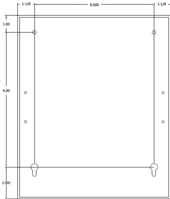
CBC Mounting Dimensions - Front View
